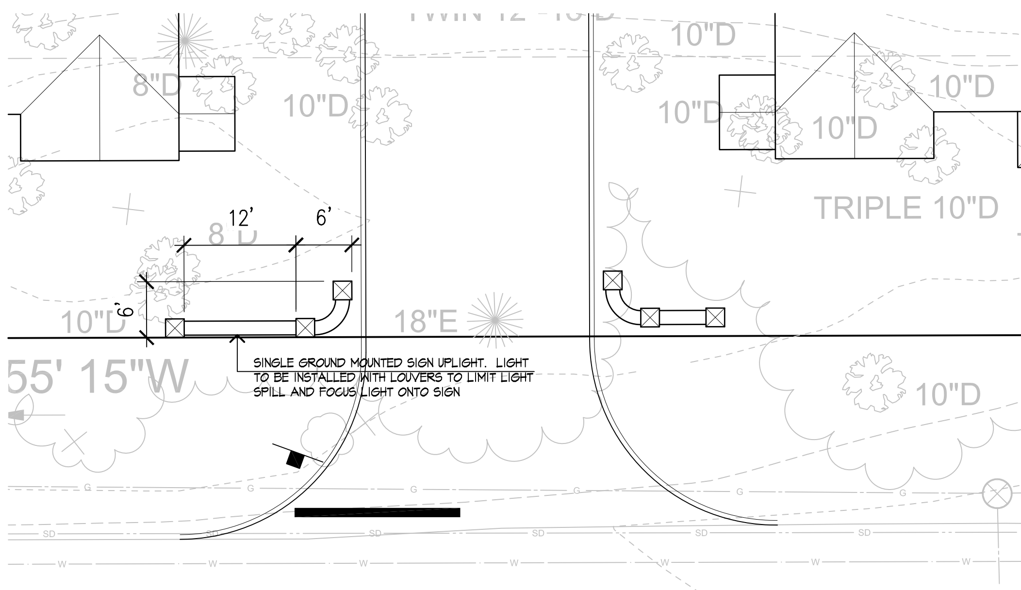
5 ENTRY MONUMENT ENLARGEMENT - PLAN SCALE: 1"=10'-0"
