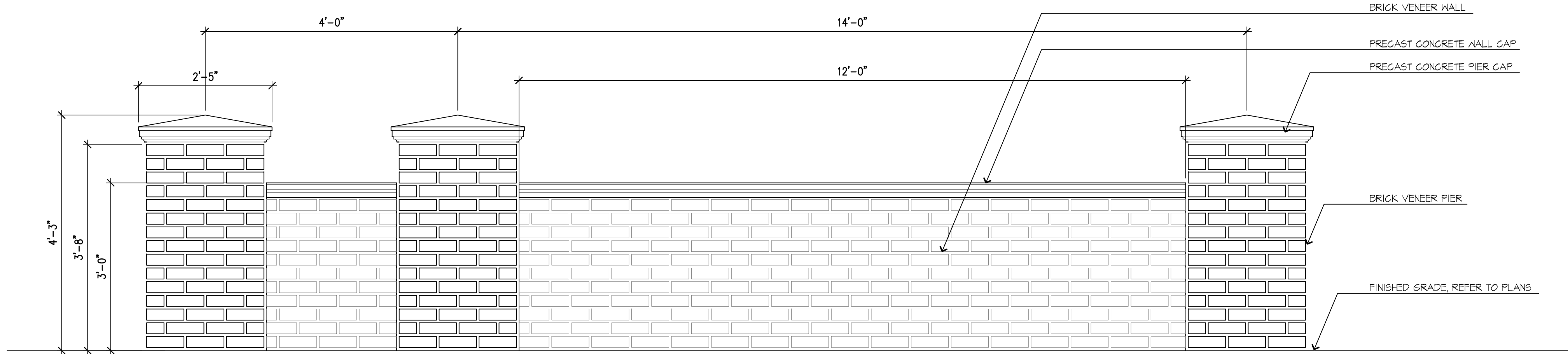
1 ENTRY MONUMENT WALL SCALE: 3/4"=1'-0"
