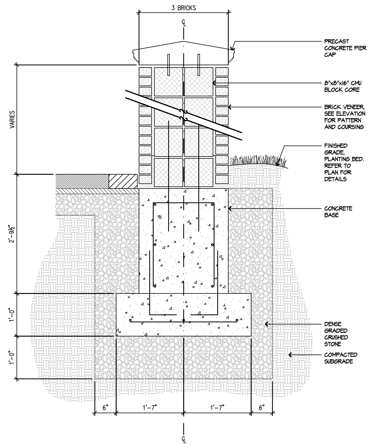
2 ENTRY MONUMENT PIER - SECTION SCALE: 3/4"=1'-0"
