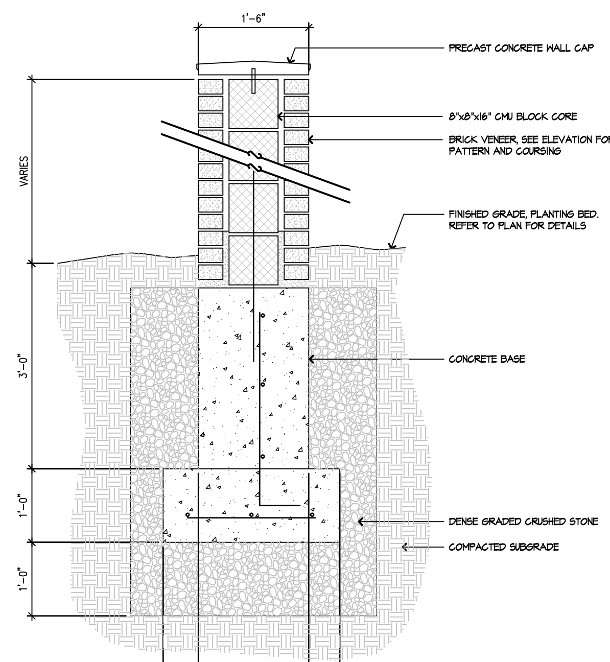
4 ENTRY MONUMENT WALL - SECTION SCALE: 3/4"=1'-0"
