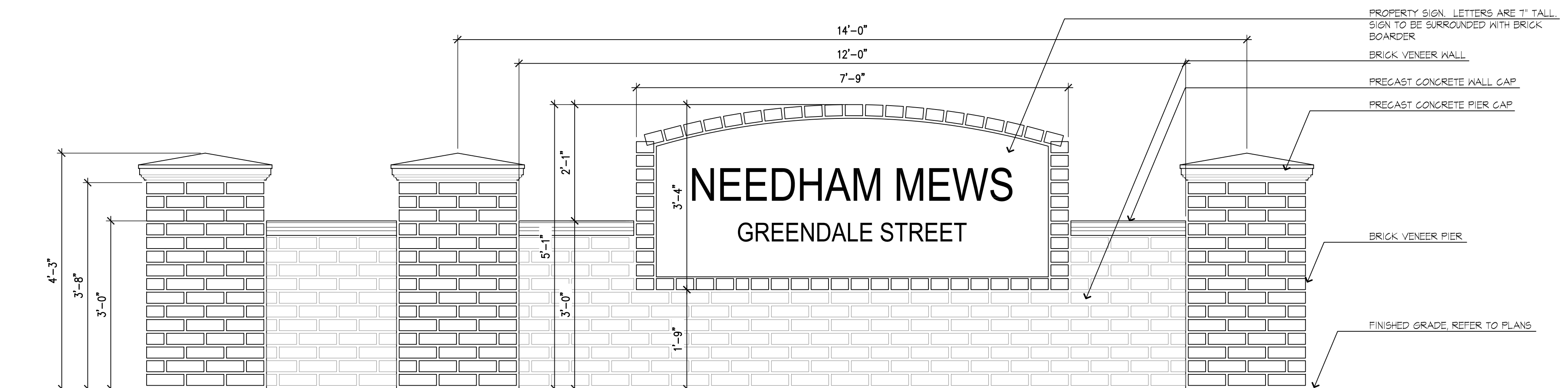
3 ENTRY MONUMENT WALL WITH PROPERTY SIGN SCALE: 3/4"=1'-0"
