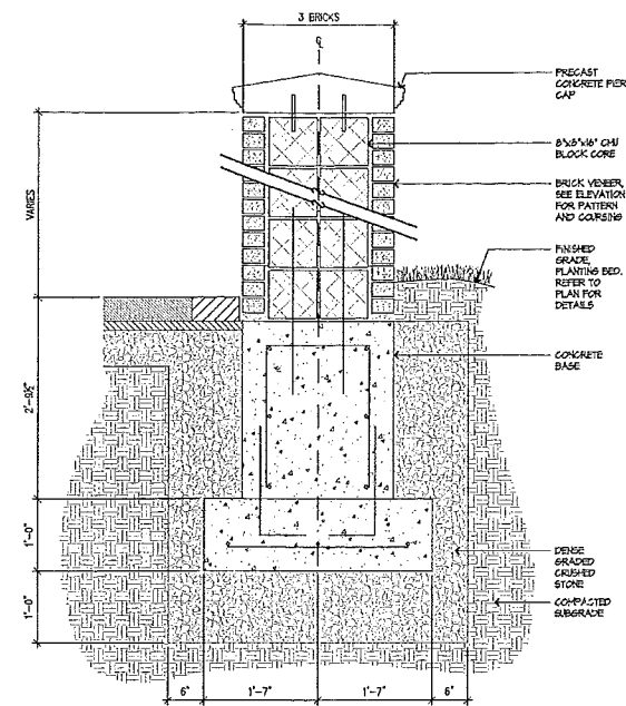
2 ENTRY MONUMENT PIER - SECTION SCALE: 3/4"=1'-0"
