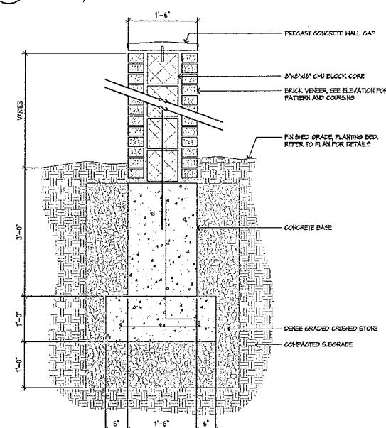
4 ENTRY MONUMENT WALL - SECTION SCALE: 3/4"=1'-0"
