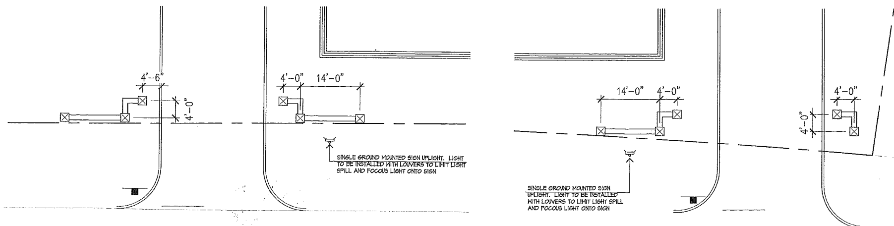
3 ENTRY MONUMENT WALL WITH PROPERTY SIGN SCALE: 3/4"=1'-0"
