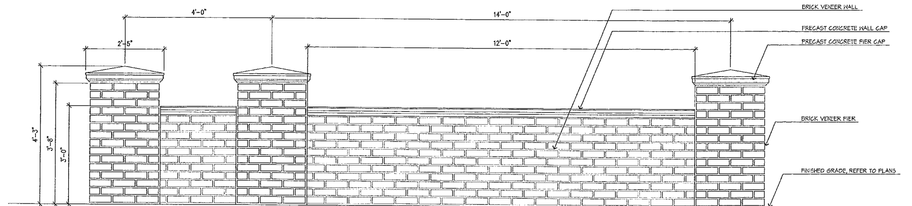
1 ENTRY MONUMENT WALL SCALE: 3/4"=1'-0"
