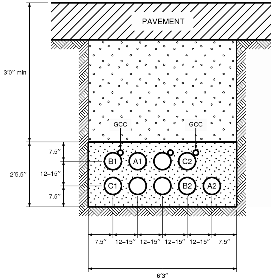
Figure 3. An as-built duct-bank section with a 2×5 arrangement of ducts designed to pass beneath existing utilities.
