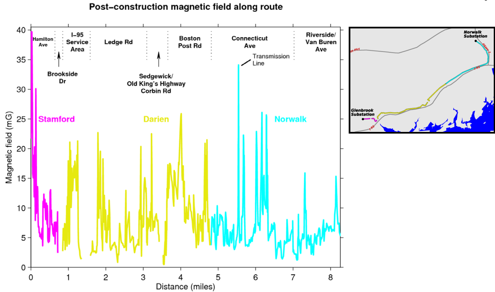
Figure 7. Post-construction measurements of magnetic fields along the project route.
