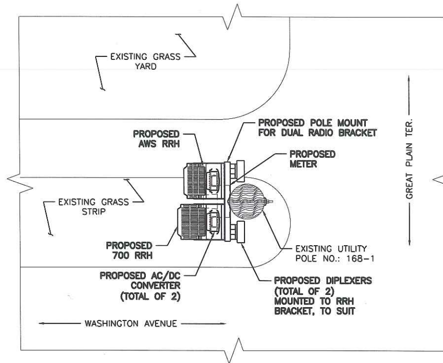
① RRH ORIENTATION PLAN 3/8" = 1'-0"
